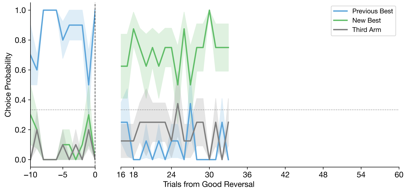
Good Reversal-Aligned Choices (mean \pm se across subjects | n=5 subjects, n=9 reversals) (Skipping first 15 trials post-reversal)
